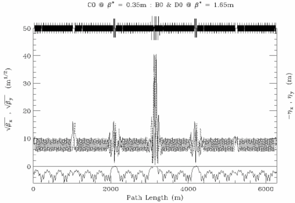
Figure 2.4: C0 collision optics – B38 → C19 (top), and ring-wide (bottom).
