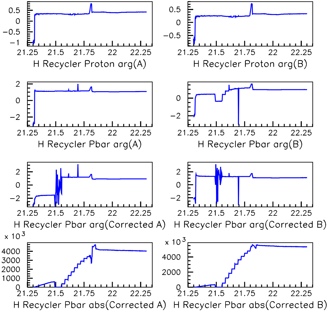
Figure 8: These plots show damper board data. The top 4 plots are the phase of the raw A and B signals from the proton and antiproton cables. The next two plots are the phase of the A and B signals, after cancellation of the proton contamination, from the Pbar cables. In all cases the phase is stable when the beam conditions are stable. The final two plots are the magnitude of the signals whose phases were plotted in the previous two plots. The magnitudes of the top 4 signals are shown in figure 1.
