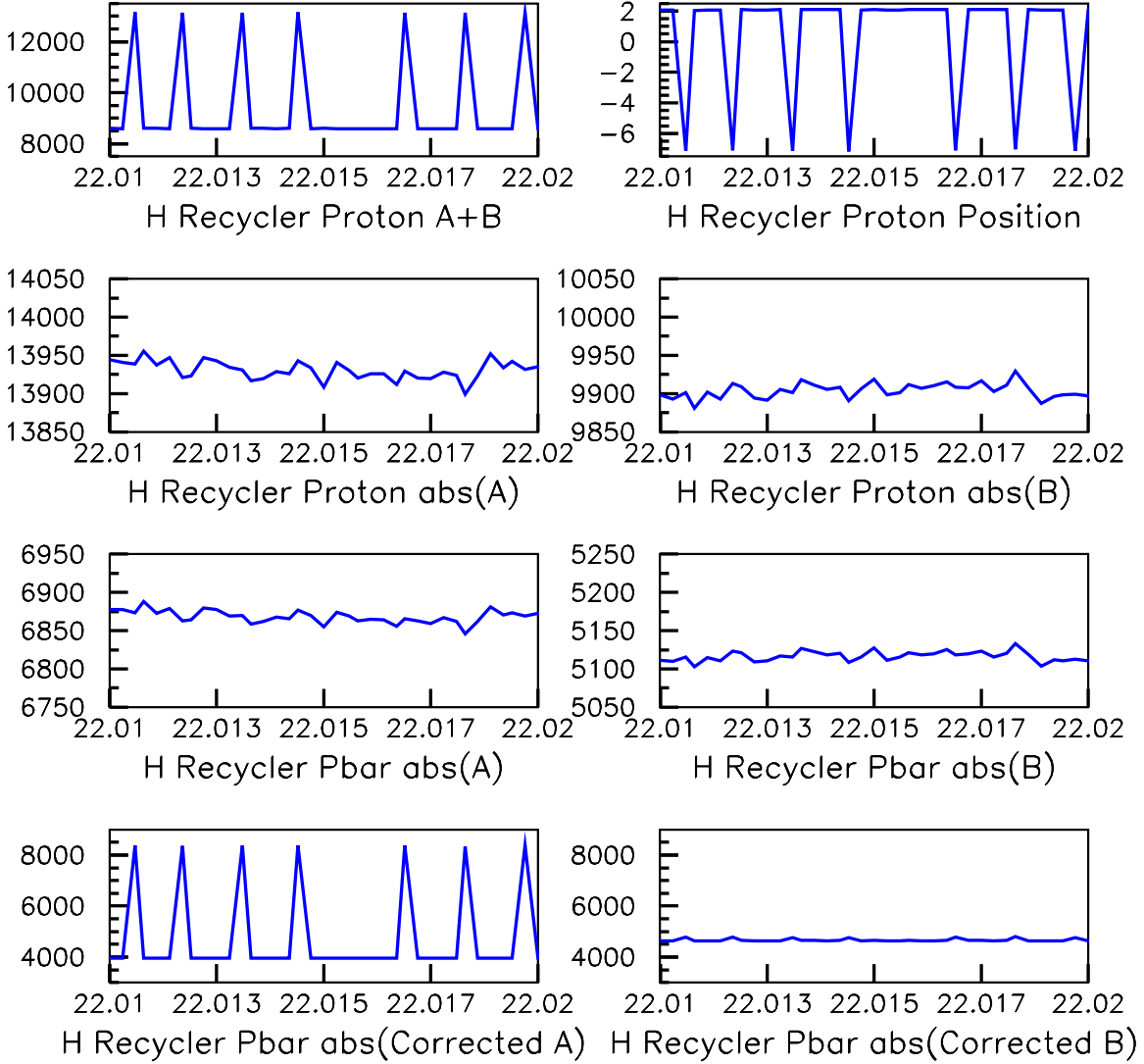
Figure 7: This figure has the same layout as figure 6 but the information plotted is the magnitude of the signals. The middle 4 plots all have different zero suppression but all 4 plots have a vertical window of 200 counts. The bottom two plots have the same vertical scale. From this we learn that the noise in the antiproton sum and position signal comes from the algorithm which removes the proton contamination on the A plate.
