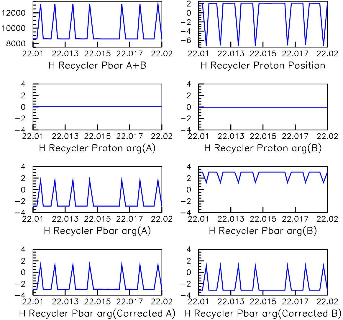
Figure 9: This figure has the same layout as figure 6 but each point has a phase rotation to make the phase of Proton A+B zero. Here we see clearly that the Pbar phases are bi-stable relative to the phase of Proton A+B.
