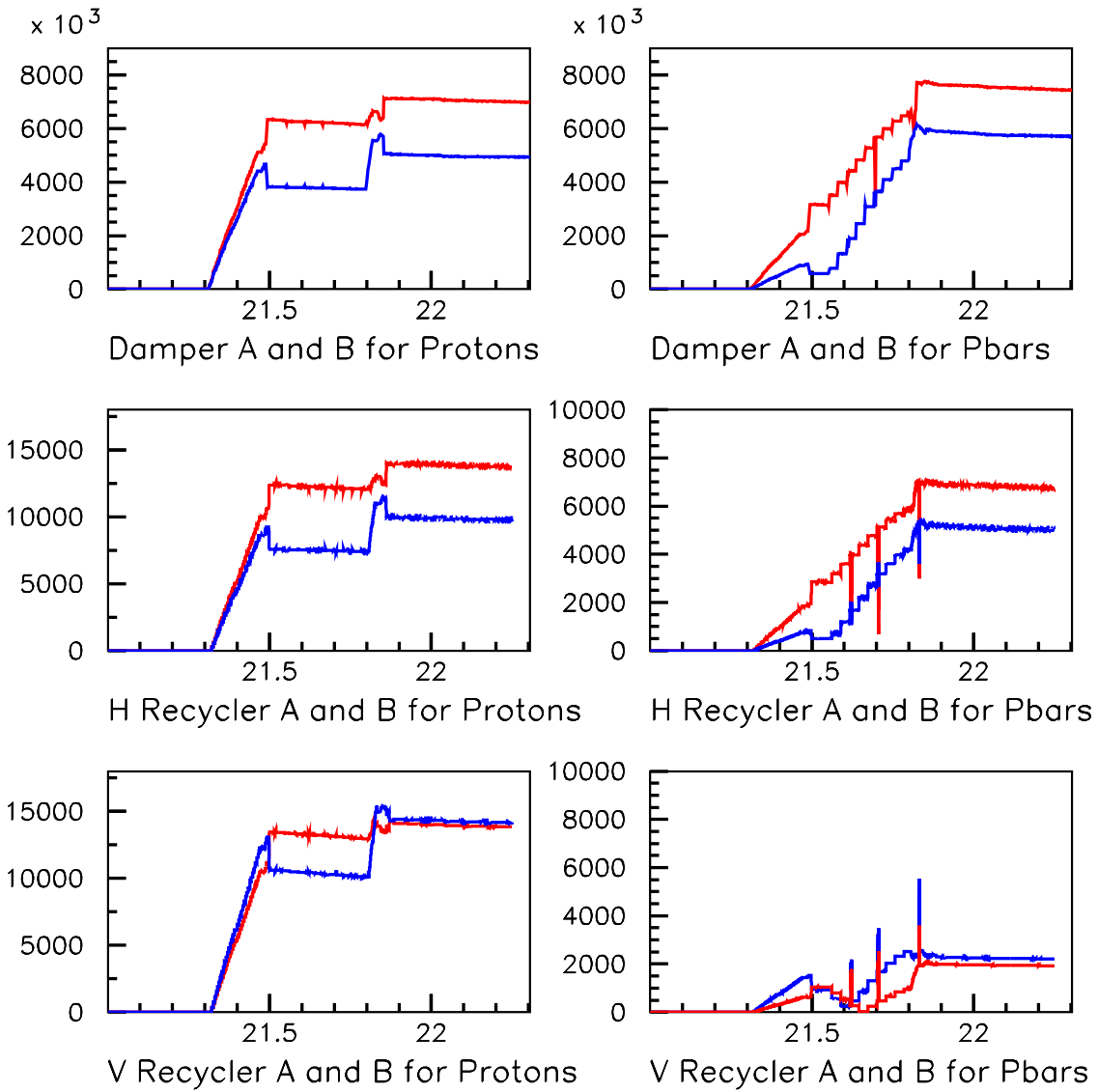
Figure 1: Raw |A| and |B| signals for protons and antiprotons, for each of the three boards.
