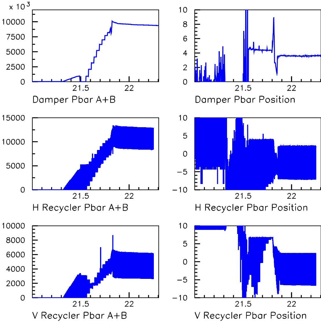
Figure 3: Antiproton sum and position signals, for each of the three boards. The proton signals on the antiproton cables were canceled as described in Beamsdoc-988.
