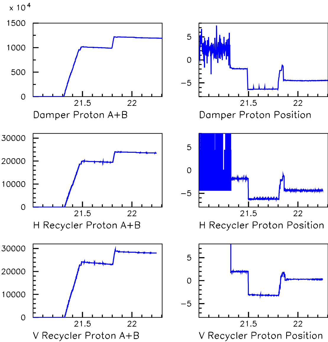
Figure 2: Proton sum and position signals, for each of the three boards.
