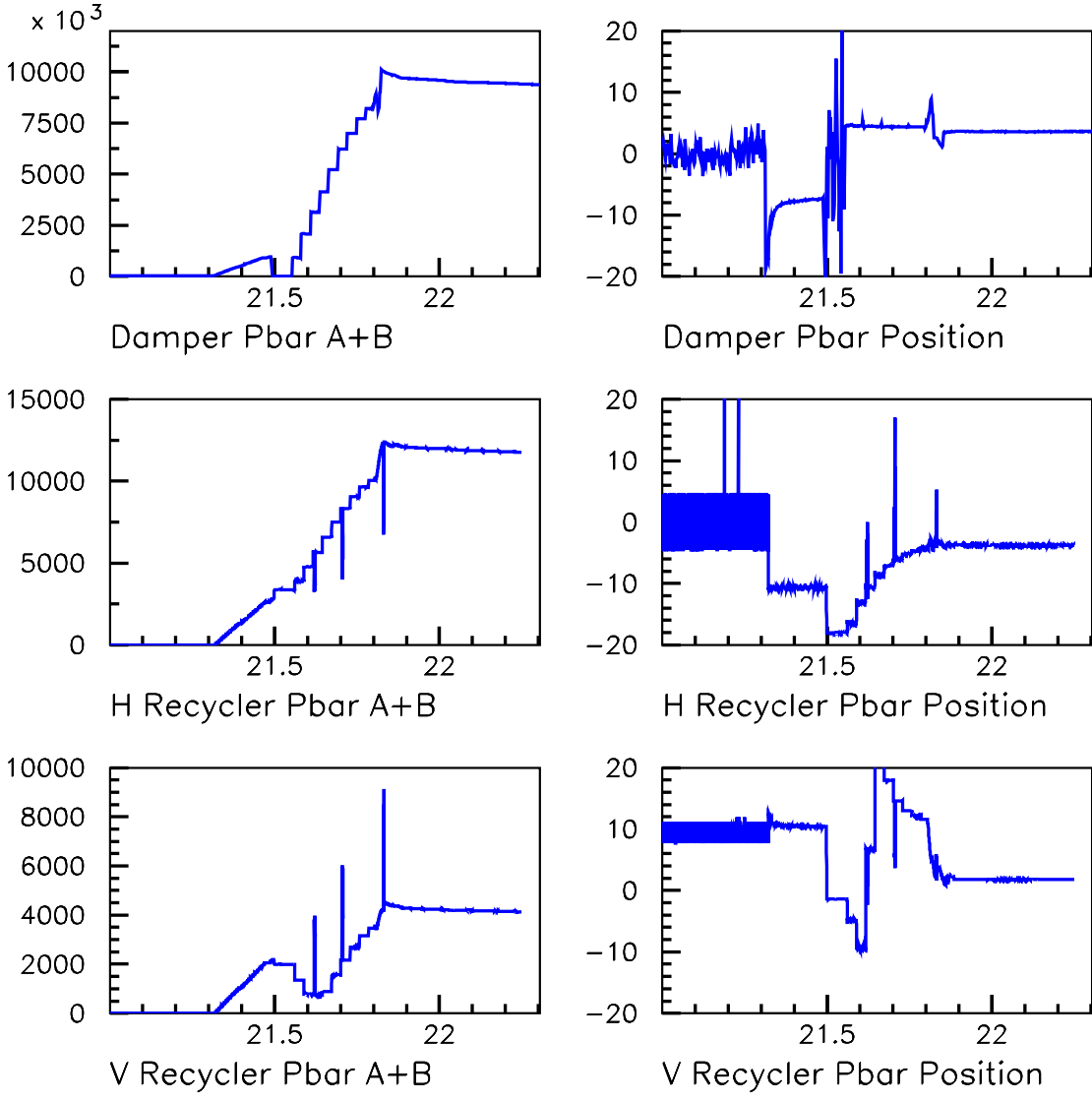
Figure 5: The damper board data is the same as figure 3. For the recycler board data, this is the same as figure 3 but without the cancellation of the proton noise on the antiproton cables.
