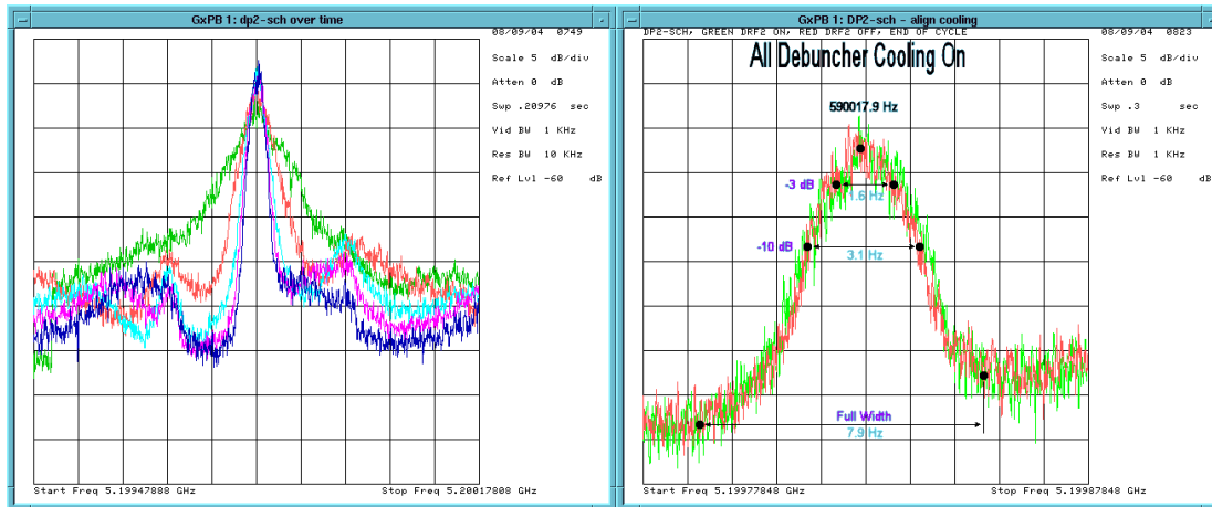
Figure 10: Debuncher Momentum band 2 cooling signal DP2-SCH over time. The green trace is taken at bunch rotation time. The other traces are taken at successively later times. The dark blue trace is taken at the end of the cycle. The plot on the right is the same signal, sampled at the end of the Debuncher cycle with the span zoomed in. Examination of traces like these could allow us to establish baselines for Debuncher beam operation.
