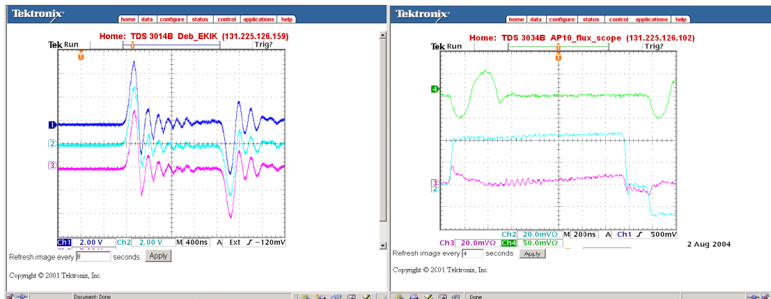
Figure 9: Network Scope Traces. The picture on the left is the Debuncher Injection Kicker Thyrotons firing. The picture on the right is the AP10 flux scope.
