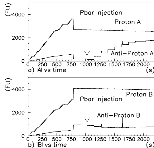
Figure 1: Magnitudes of the raw signals on the four channels from the BPM HB34. The time axis is in seconds from the start of the data set. The vertical axis is in Echotek units.
