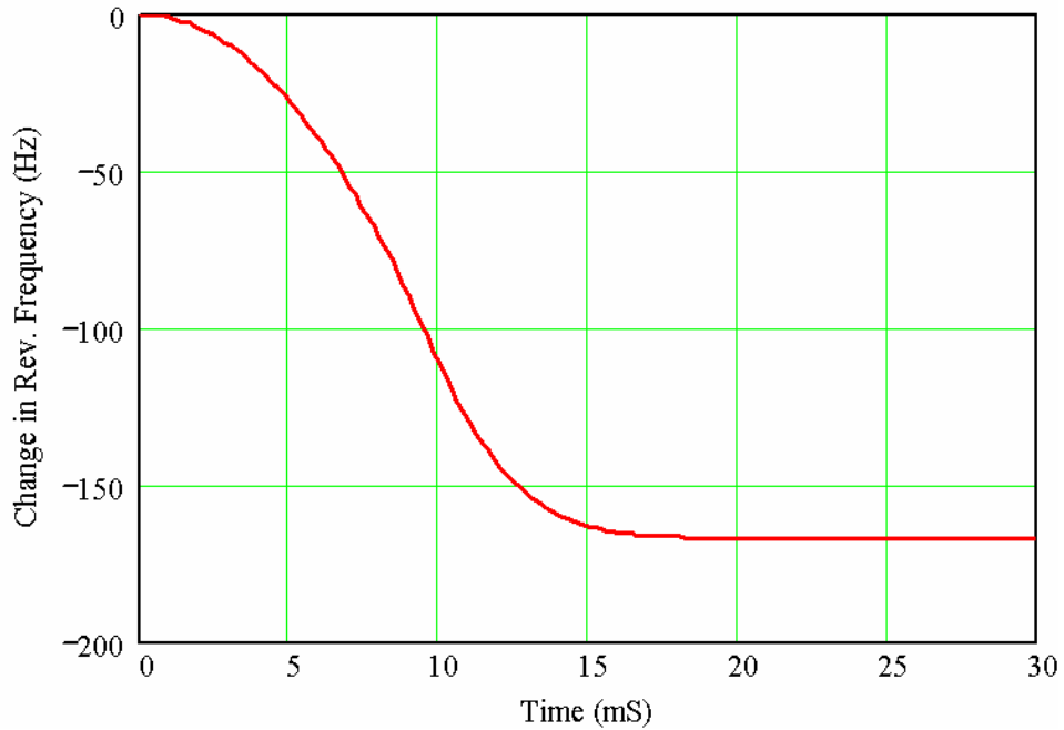
Figure 4-4 53 MHz Relative revolution frequency during momentum stacking. The first 10 mS of the curve is a second order polynomial and the second 10 mS of the curve is a fourth order polynomial.
