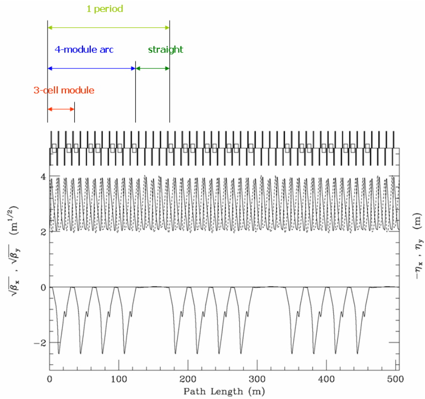
Figure 5-2 Lattice functions of the new booster
