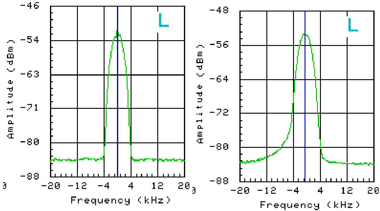
Figure 2: Digitized 1.75 GHz Schottky signals at the low intensity of 0.088 \times 10^{11} protons. Comparison of the center of the initial signal at 11.41 (left) and the peak of the final signal at 12:27 (right) gives a shift of the revolution frequency of 0.024 Hz or 0.031 Hz per hour. Energy loss per particle is 0.36 MeV/hr or 1.11 meV/turn.
