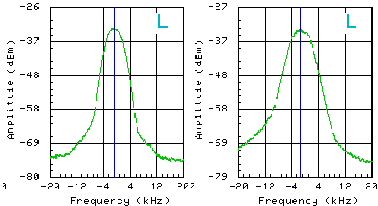
Figure 1: Digitized Schottky signals of the 19485th revolution harmonic (1.75 GHz). Comparison of the center of the initial signal at 12:29 (left) and that of the final signal at 13:30 (right) gives a shift of the revolution frequency of 0.032 Hz.
