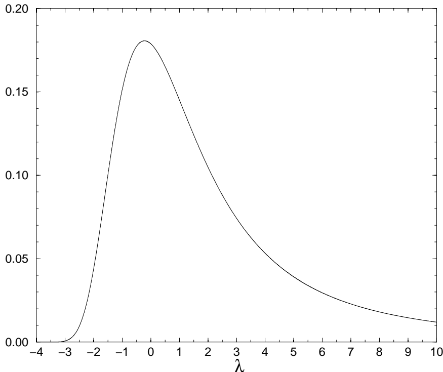
Figure 4: The Landau distribution \varphi(\lambda) . The distribution is skew and has a long tail for larger energy loss (larger \lambda ). The distribution peaks at \lambda = -0.223 and has a full-width-at-half-maximum of \lambda_{\text{FWHM}} = 2.6 .
