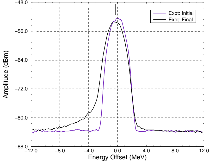
Figure 3: (color) Initial beam energy distribution (purple) centered at zero versus final beam energy distribution (black) peaked at -0.275 MeV as indicated by the black vertical bar above the distributions.
