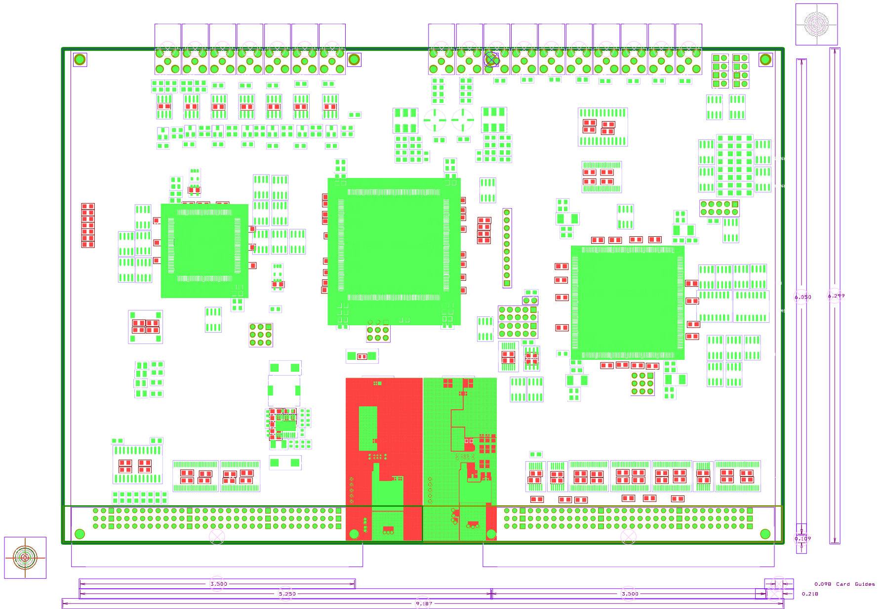
VME RF TIMER BOARD OUTLINE W/ COMPONENT PLACEMENT
