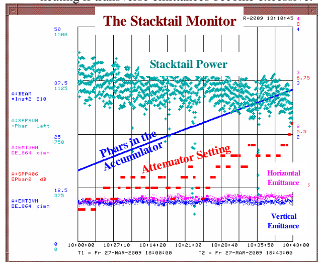
Figure 2: Stacktail Monitor Operation
