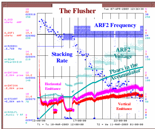
Figure 3: The Flusher controls ARF2 for stacks > 80E10.
